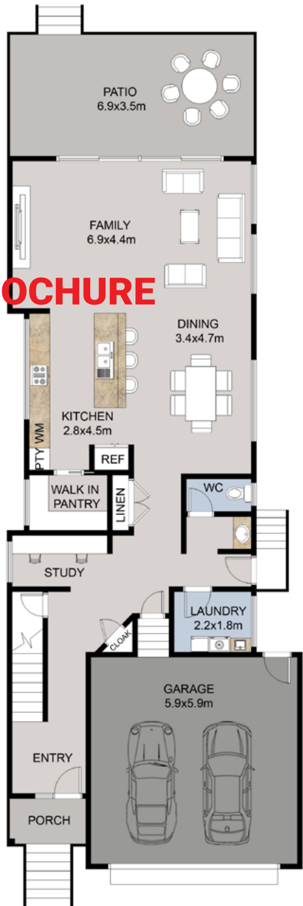
LOWER FLOOR
